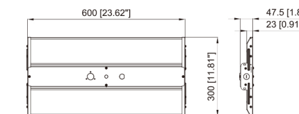
ELSLHB02 2FT 80W / 110W / 165W
